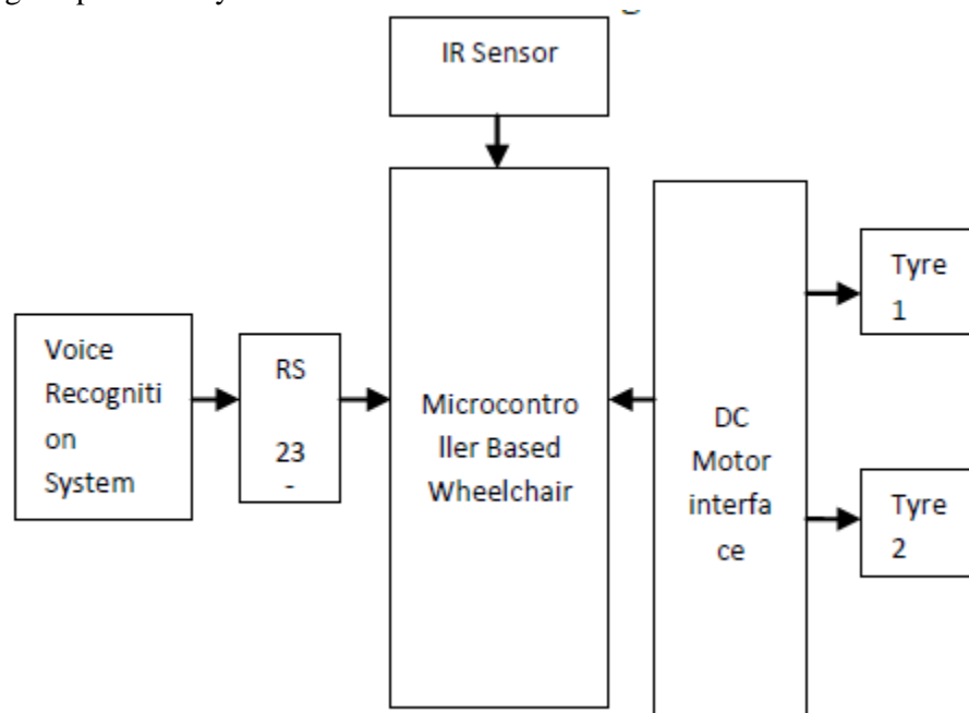
Fig.1. Block Diagram of voice operated intelligent wheelchair
