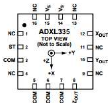
Fig.4. ADXL 335 Pin Configuration.
