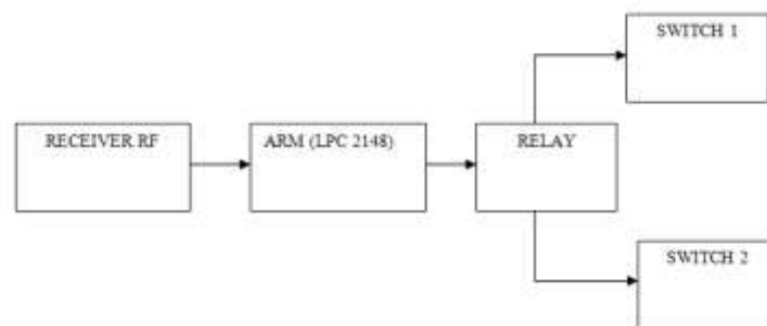
Fig.2. Remote control
