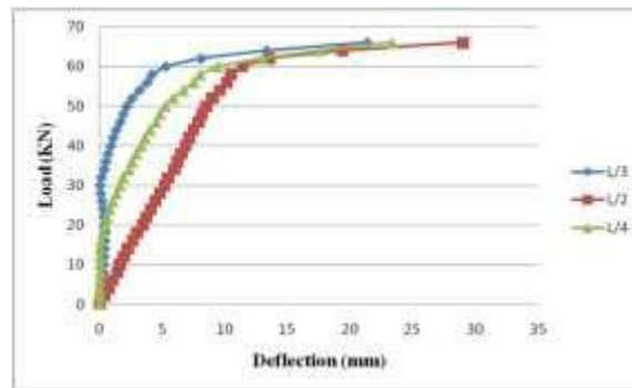
Fig.1 Load Vs Deflection Curve for Specimen SP 1
