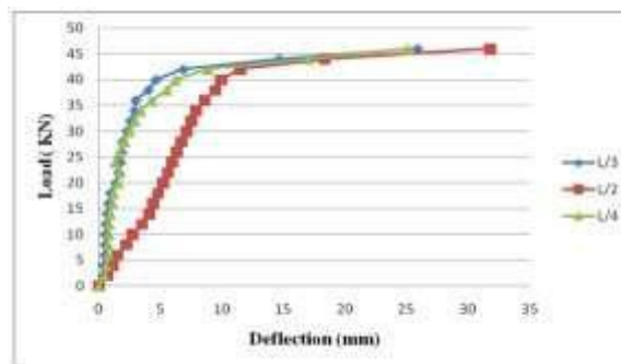
Fig.5 Load Vs Deflection Curve for Specimen SP 5
