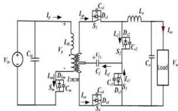
Fig.2.Zeta Converter
