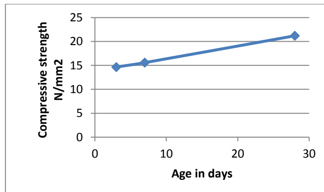
Graph 2 Compressive Strength of 5% Lime Sludge
