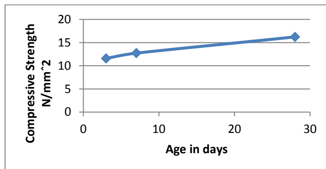
Graph 4 Compressive Strength of 15 % Lime Sludge
