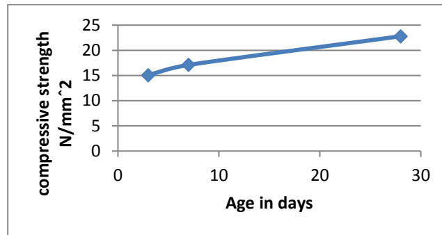
Graph 1 Compressive Strength of Normal Concrete
