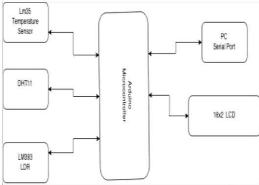
Fig. 7: Architecture Diagram
