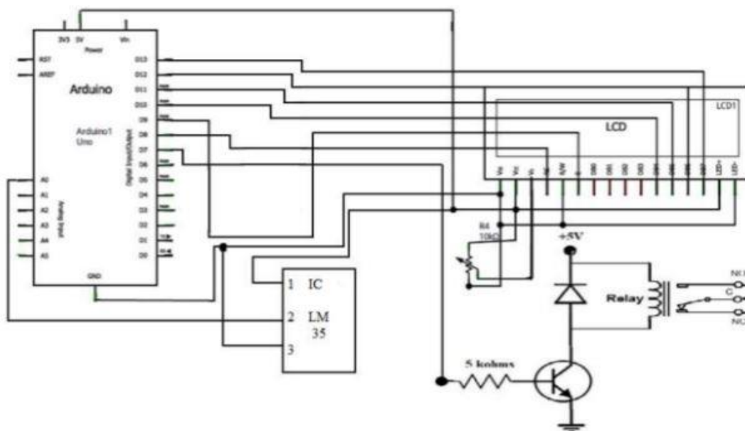
Fig 1: Circuit Diagram
